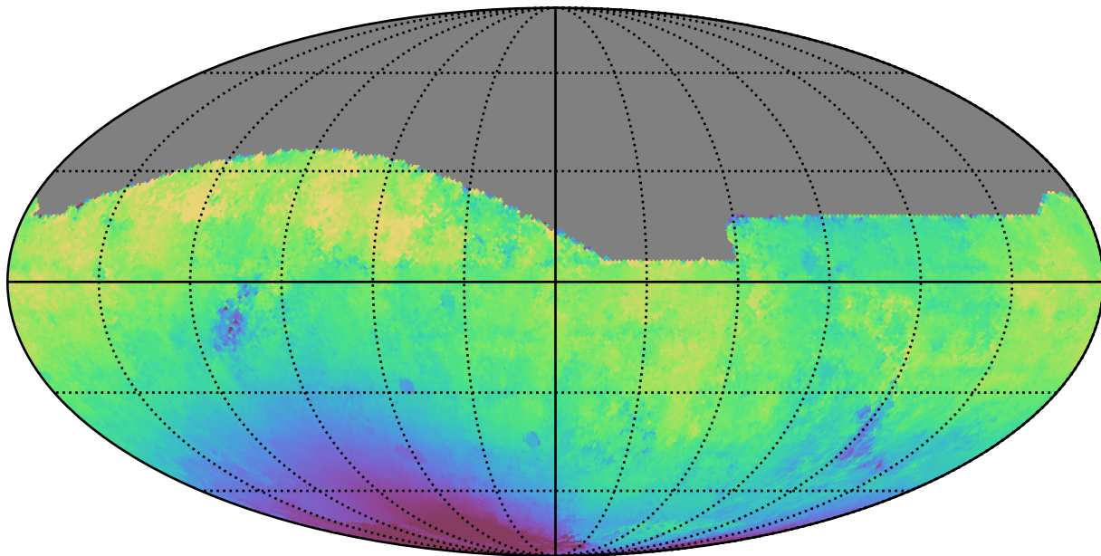
baseline_v3.5_10yrs All sky r band: Median solarElong
