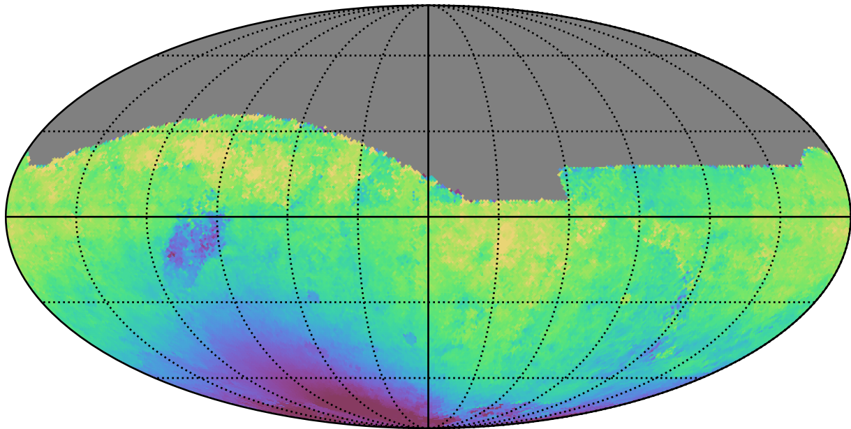
baseline_v3.5_10yrs All sky i band: Median solarElong
