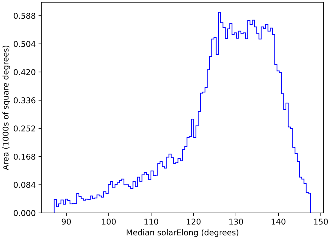
baseline_v3.5_10yrs All sky i band: Median solarElong
