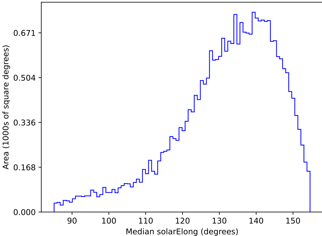
baseline_v3.5_10yrs All sky g band: Median solarElong
