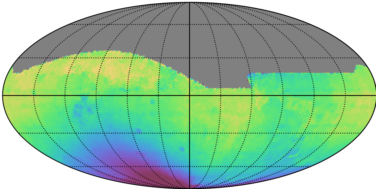
baseline_v3.5_10yrs All sky all bands: Median solarElong
