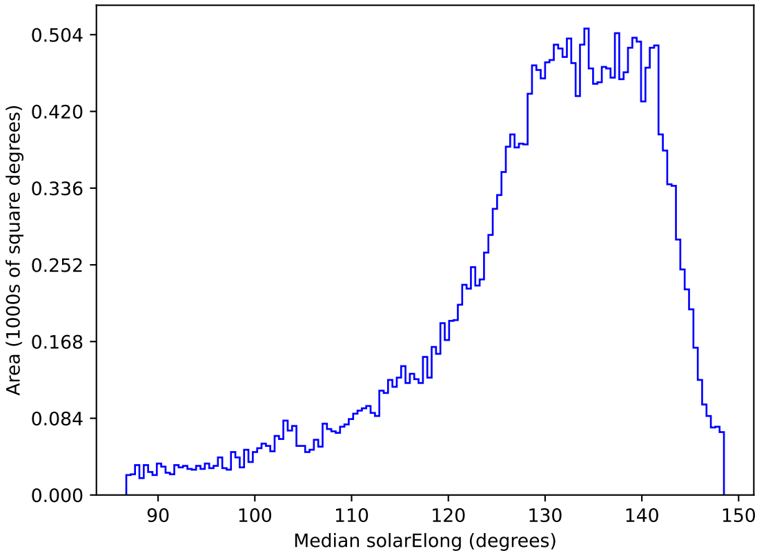
baseline_v3.5_10yrs All sky all bands: Median solarElong
