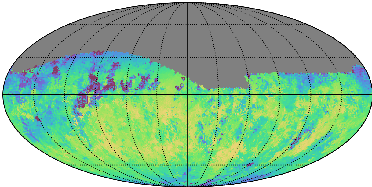
baseline_v3.5_10yrs Yr 1 z band: Median skyBrightness
