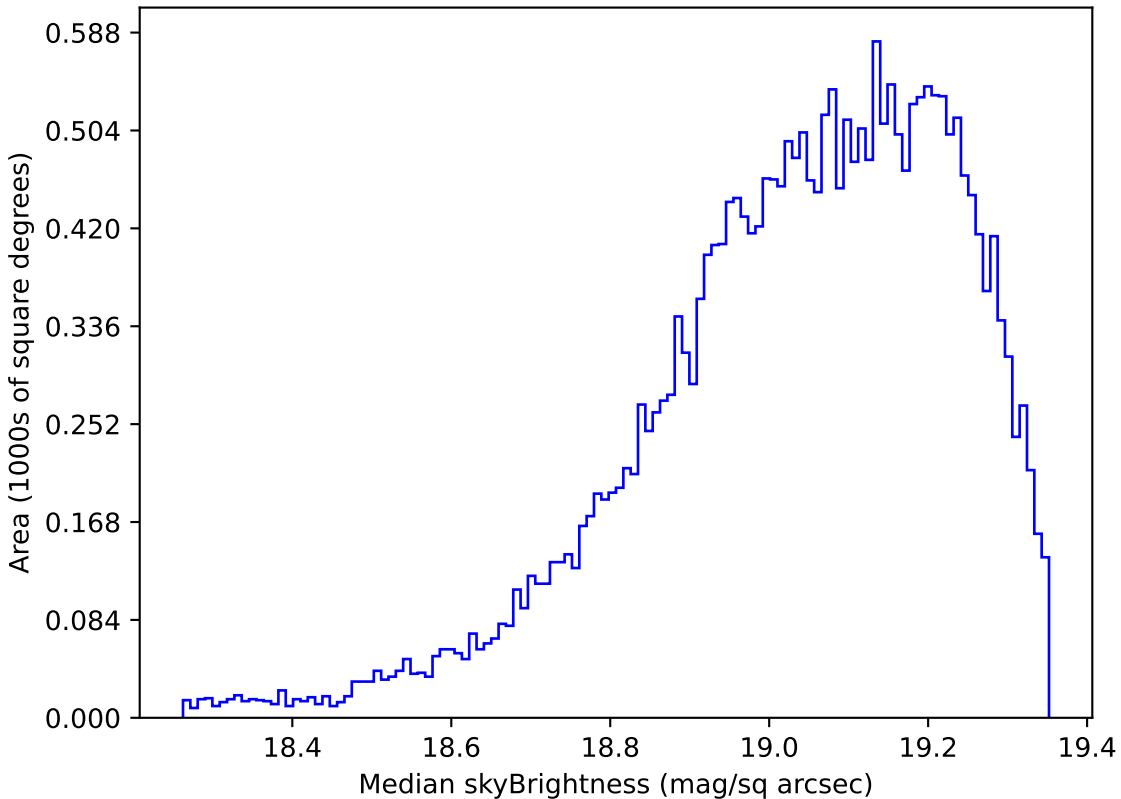
baseline_v3.5_10yrs Yr 1 z band: Median skyBrightness
