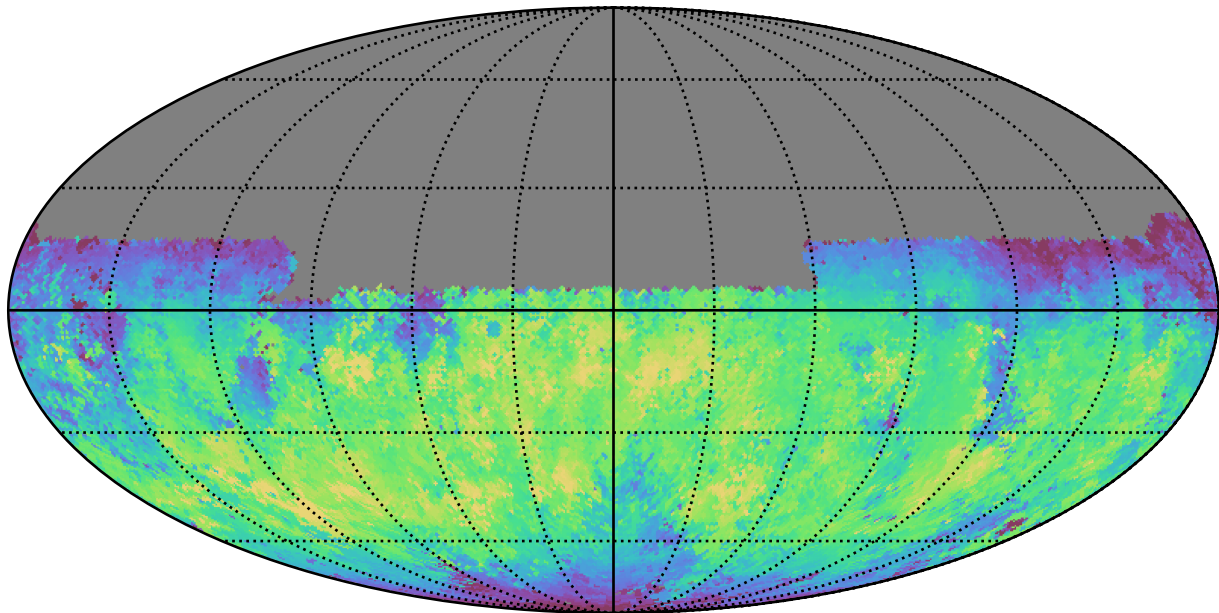
baseline_v3.5_10yrs Yr 1 y band: Median skyBrightness
