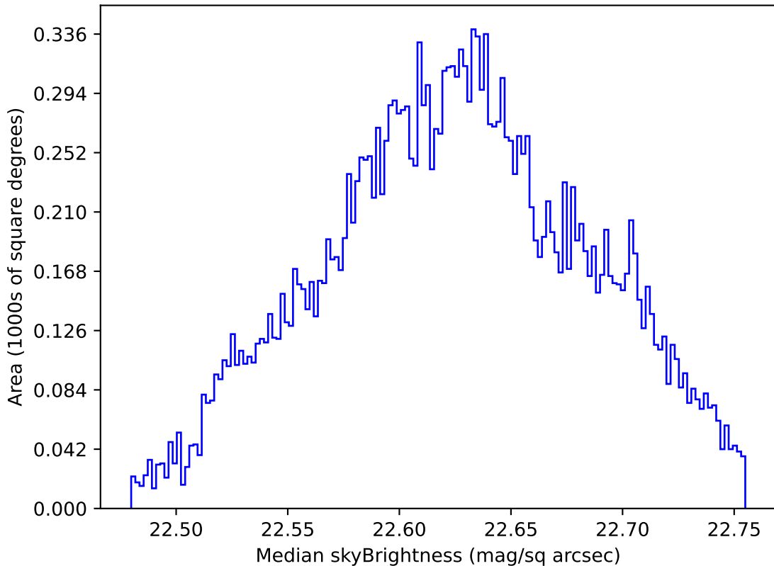
baseline_v3.5_10yrs Yr 1 u band: Median skyBrightness
