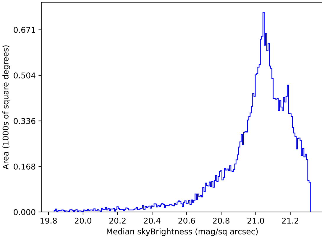
baseline_v3.5_10yrs Yr 1 r band: Median skyBrightness
