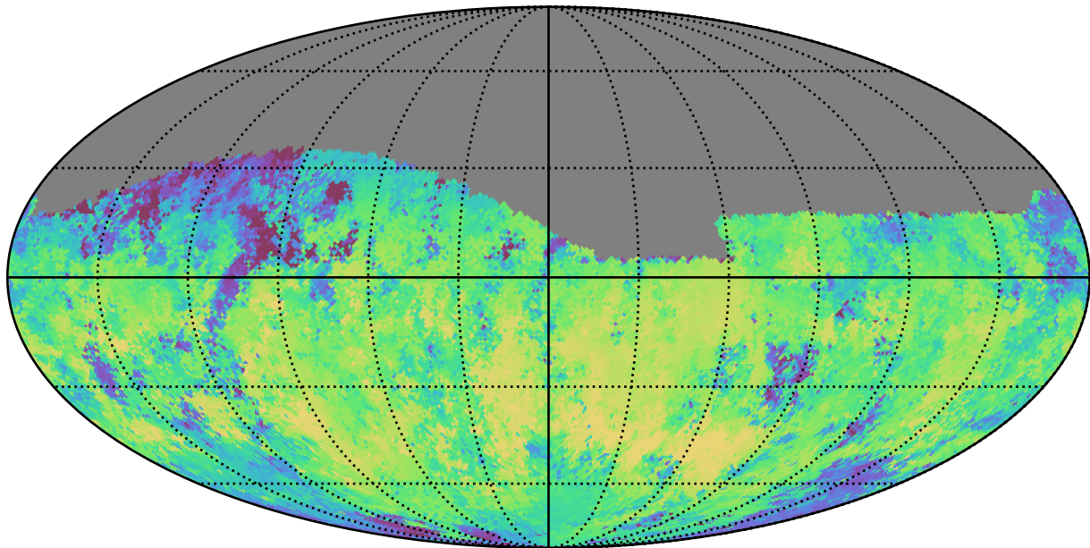
baseline_v3.5_10yrs Yr 1 i band: Median skyBrightness
