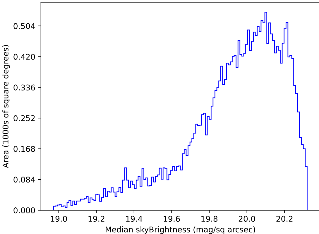
baseline_v3.5_10yrs Yr 1 i band: Median skyBrightness
