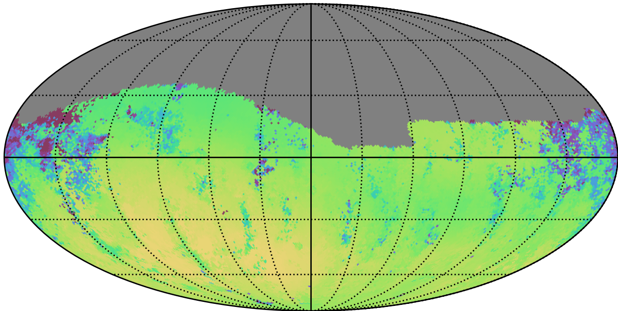
baseline_v3.5_10yrs Yr 1 g band: Median skyBrightness
