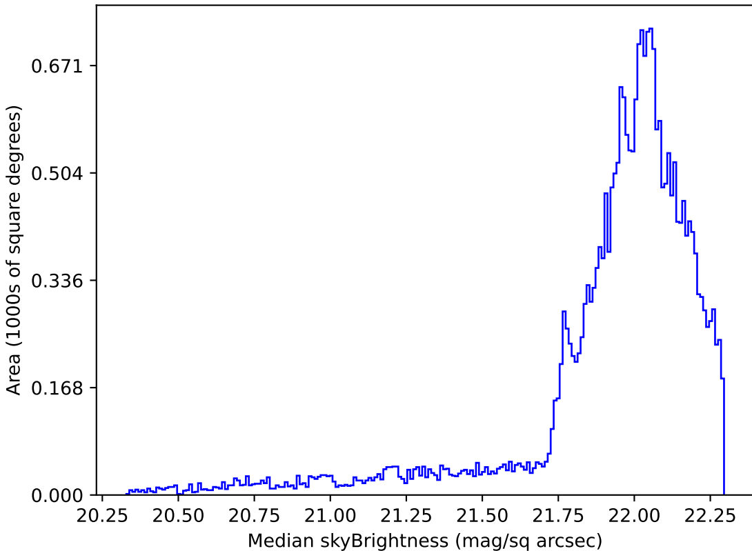
baseline_v3.5_10yrs Yr 1 g band: Median skyBrightness
