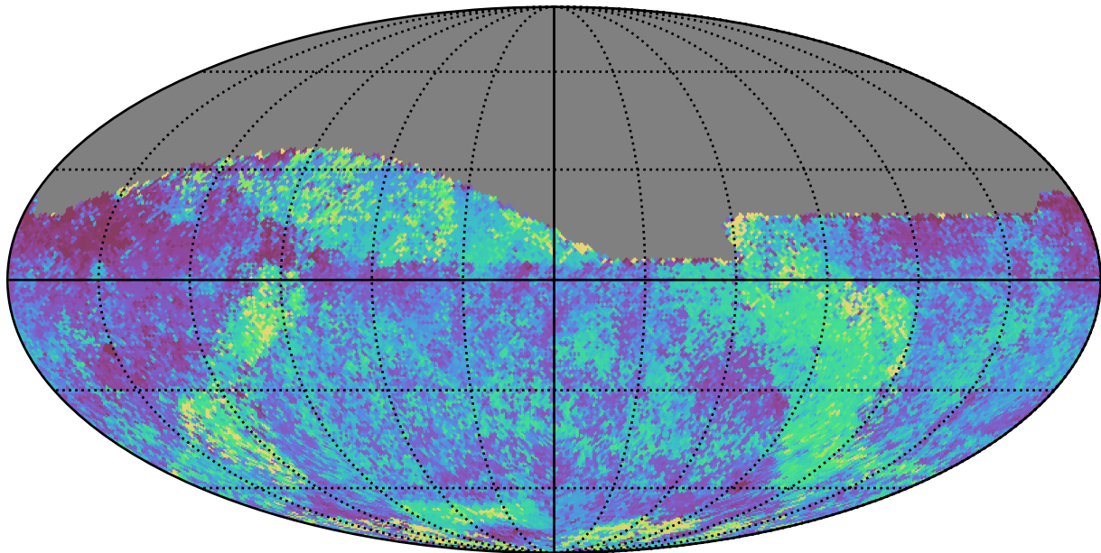
baseline_v3.5_10yrs Yr 1 all bands: Median skyBrightness
