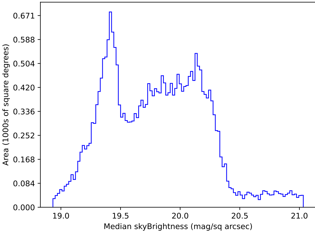
baseline_v3.5_10yrs Yr 1 all bands: Median skyBrightness
