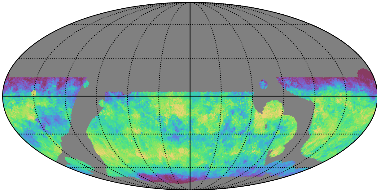
baseline_v3.5_10yrs WFD z band: Median skyBrightness
