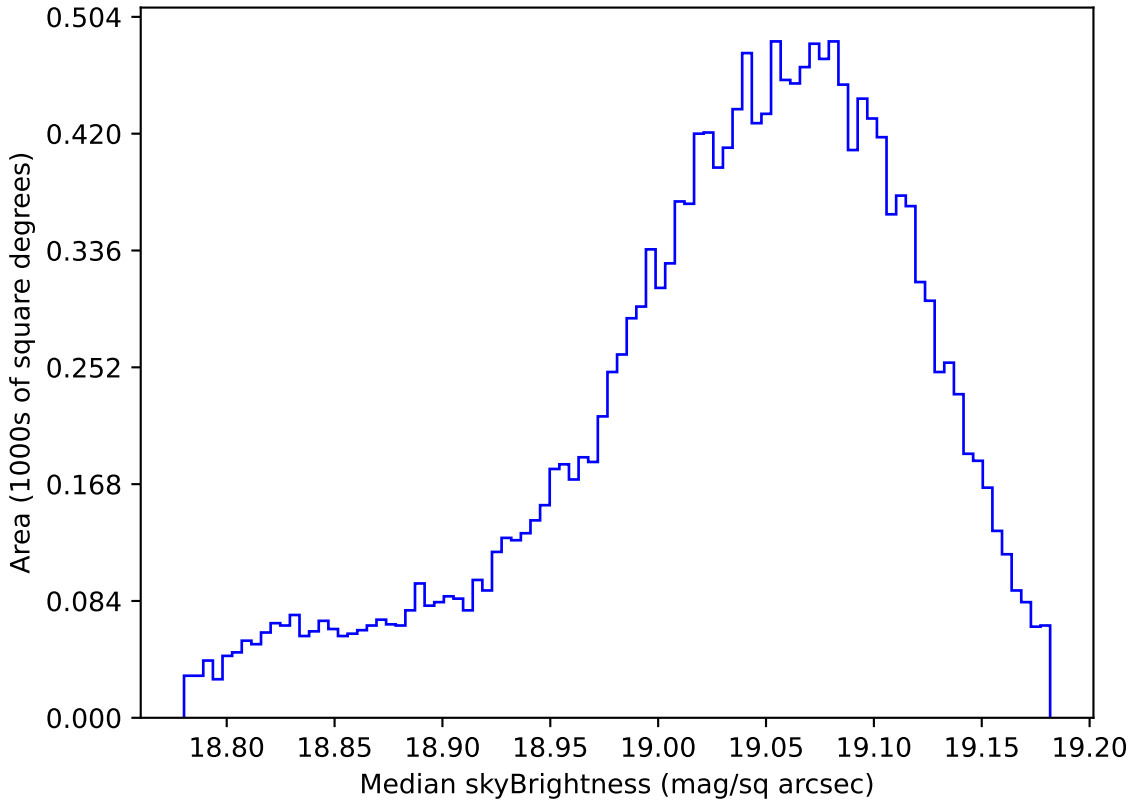
baseline_v3.5_10yrs WFD z band: Median skyBrightness
