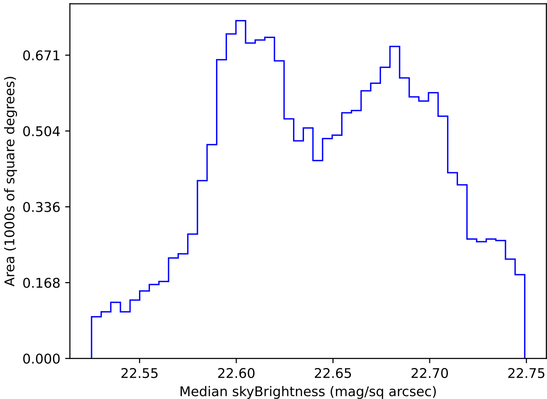
baseline_v3.5_10yrs WFD u band: Median skyBrightness
