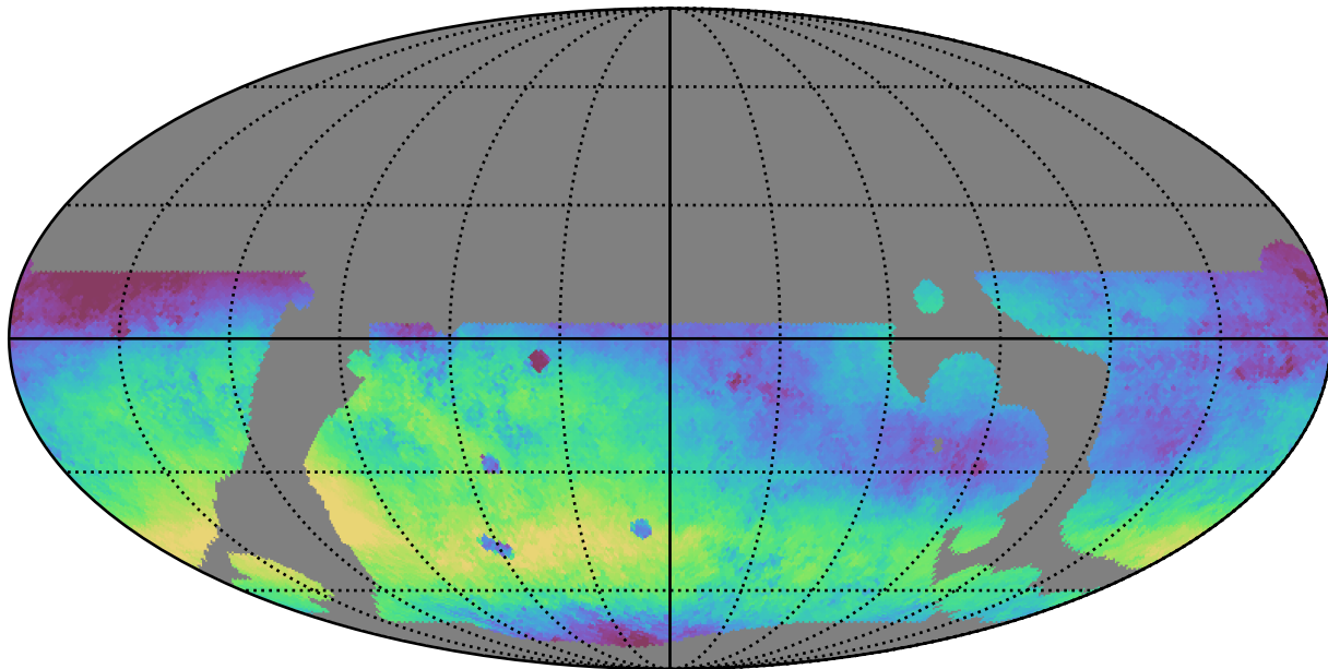
baseline_v3.5_10yrs WFD r band: Median skyBrightness
