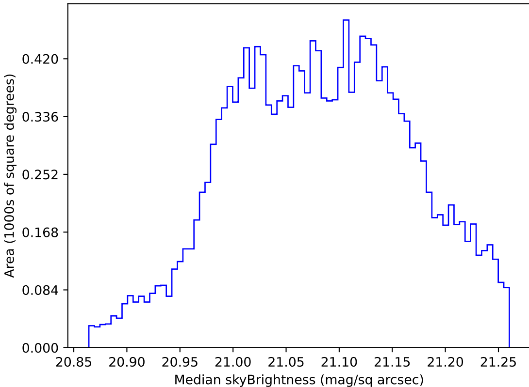
baseline_v3.5_10yrs WFD r band: Median skyBrightness
