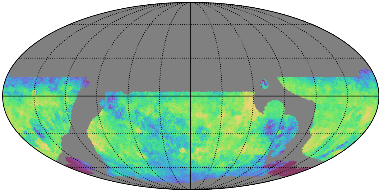
baseline_v3.5_10yrs WFD i band: Median skyBrightness
