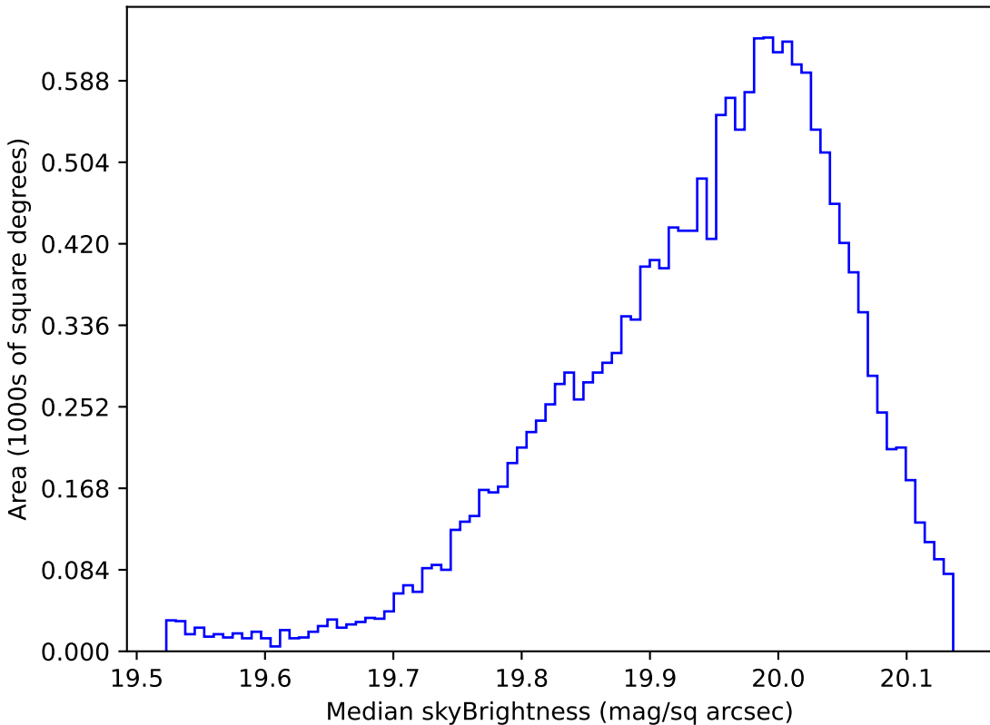
baseline_v3.5_10yrs WFD i band: Median skyBrightness
