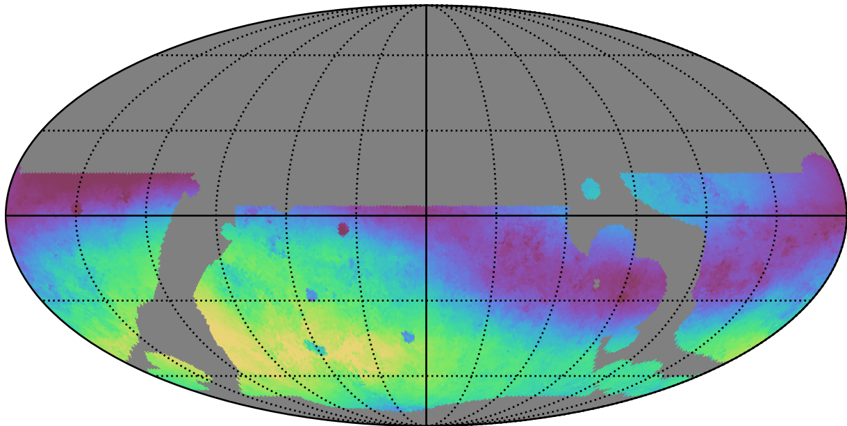
baseline_v3.5_10yrs WFD g band: Median skyBrightness
