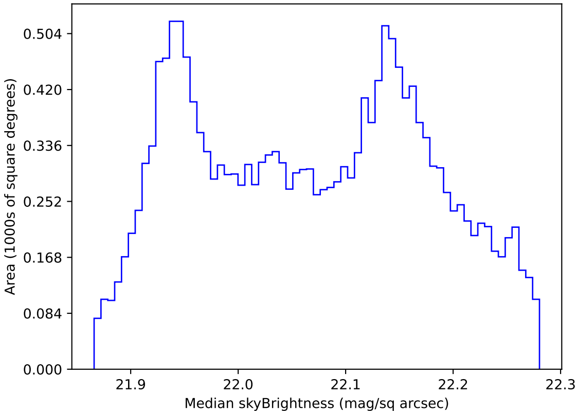
baseline_v3.5_10yrs WFD g band: Median skyBrightness
