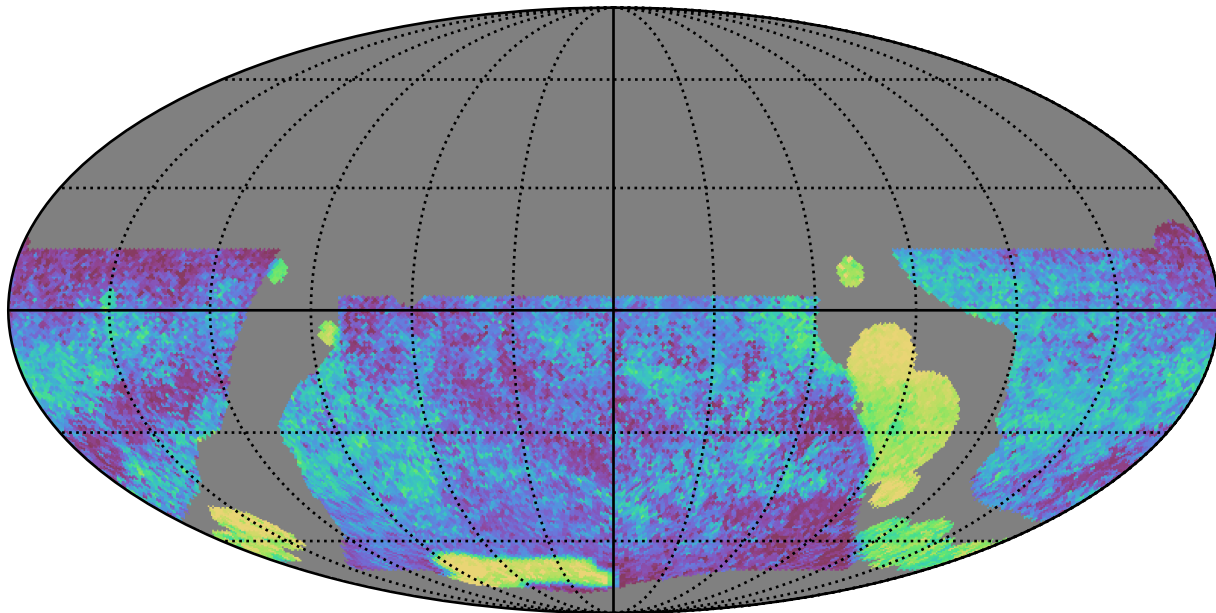
baseline_v3.5_10yrs WFD all bands: Median skyBrightness
