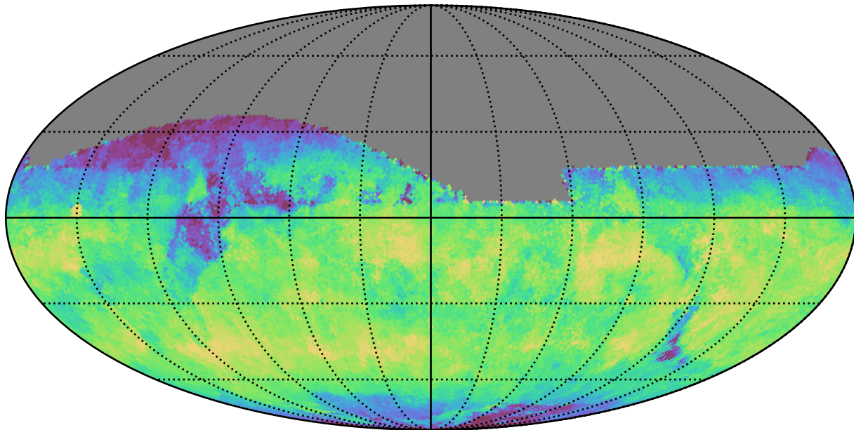
baseline_v3.5_10yrs All sky z band: Median skyBrightness
