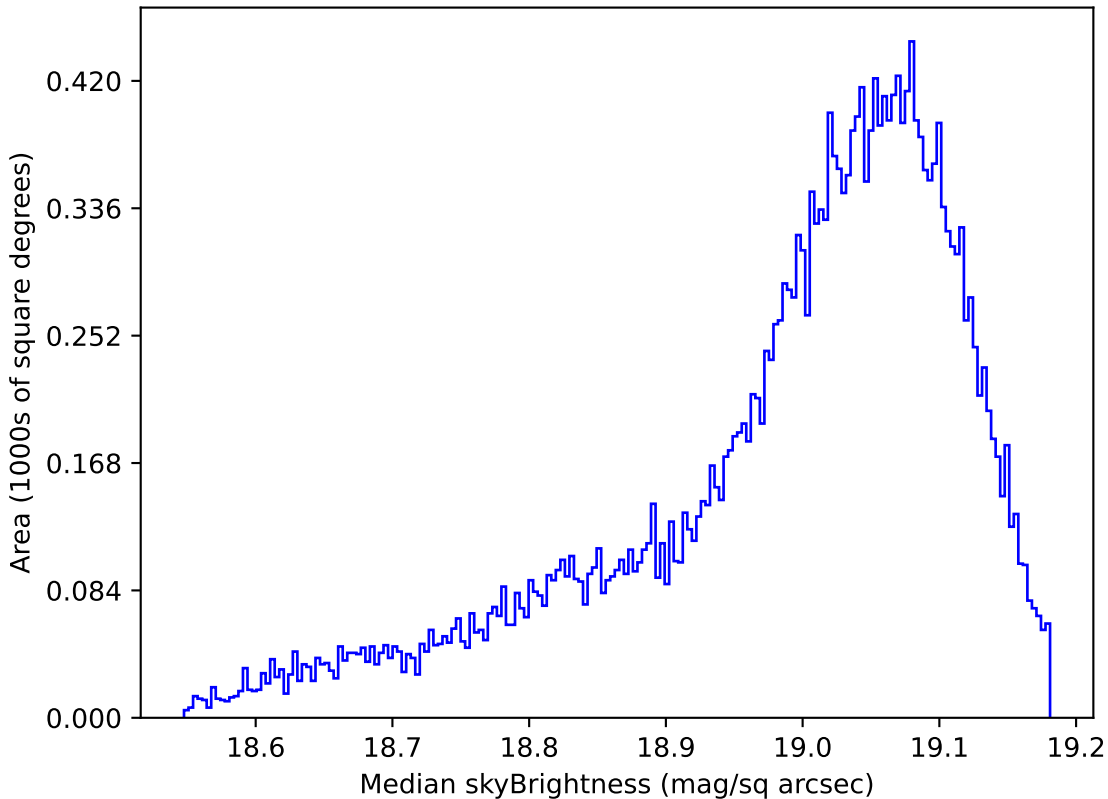
baseline_v3.5_10yrs All sky z band: Median skyBrightness
