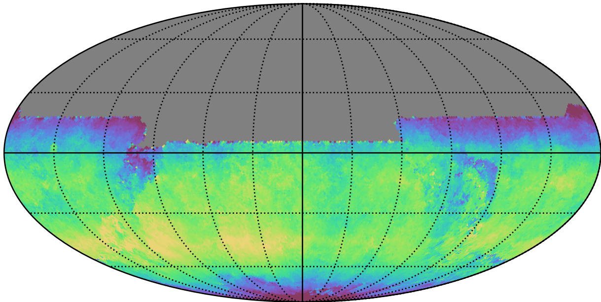
baseline_v3.5_10yrs All sky y band: Median skyBrightness
