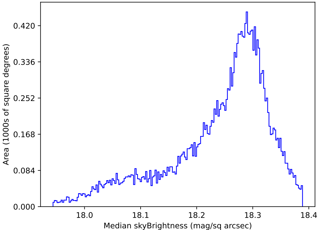
baseline_v3.5_10yrs All sky y band: Median skyBrightness
