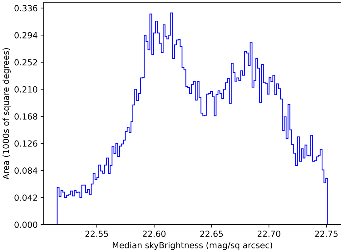
baseline_v3.5_10yrs All sky u band: Median skyBrightness
