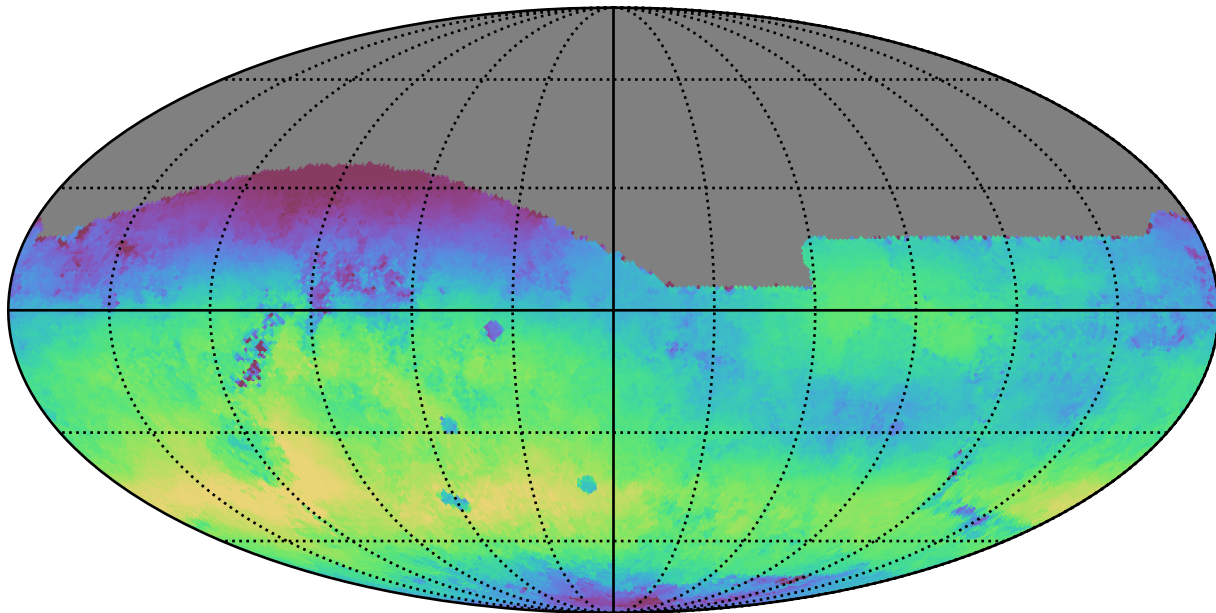
baseline_v3.5_10yrs All sky r band: Median skyBrightness
