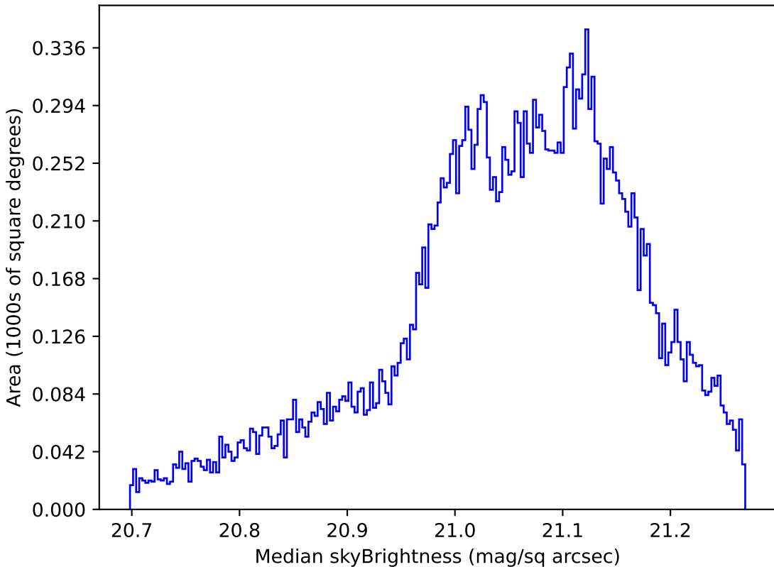
baseline_v3.5_10yrs All sky r band: Median skyBrightness
