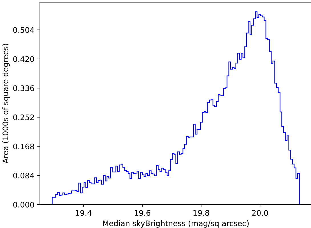
baseline_v3.5_10yrs All sky i band: Median skyBrightness
