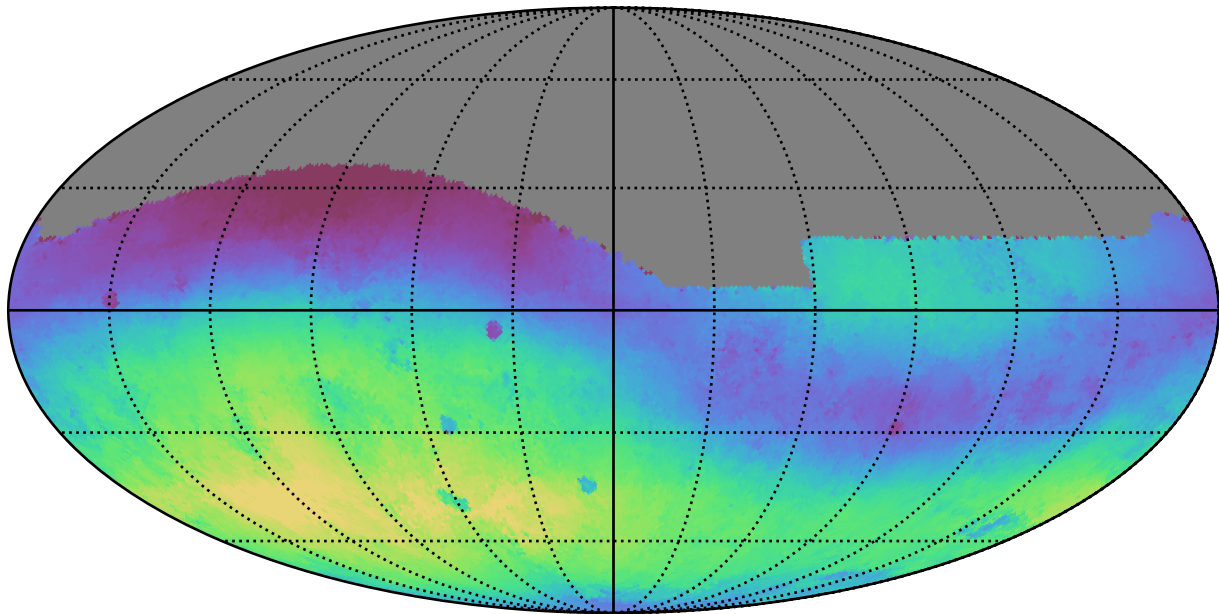
baseline_v3.5_10yrs All sky g band: Median skyBrightness
