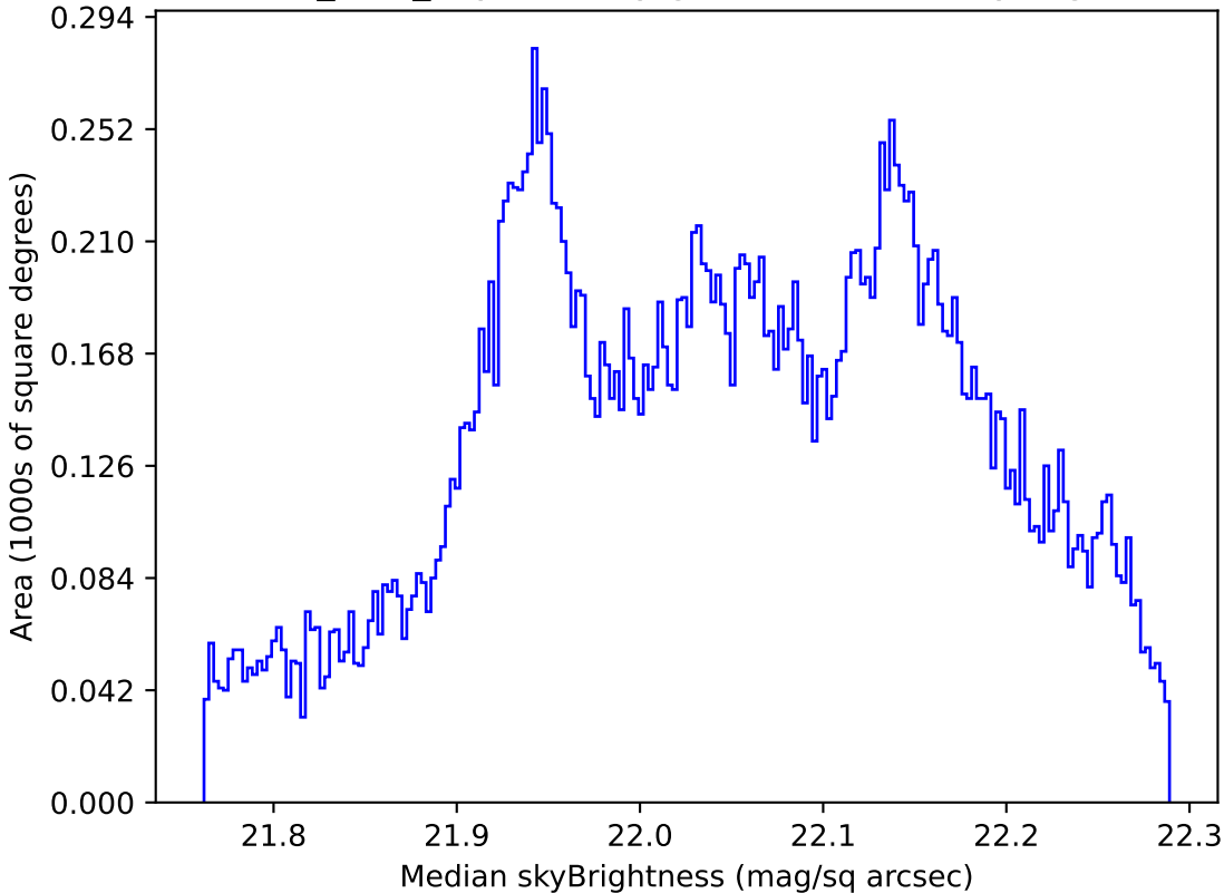
baseline_v3.5_10yrs All sky g band: Median skyBrightness
