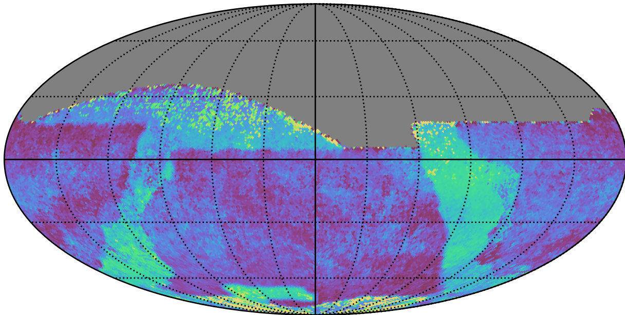
baseline_v3.5_10yrs All sky all bands: Median skyBrightness
