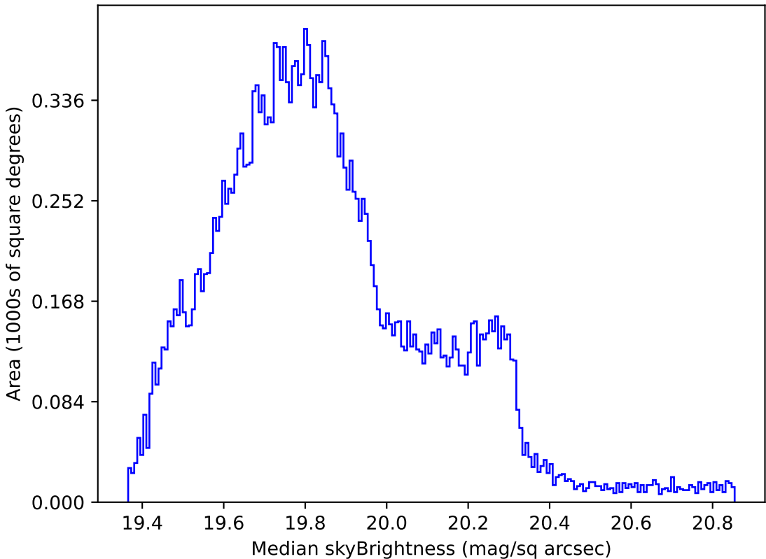
baseline_v3.5_10yrs All sky all bands: Median skyBrightness
