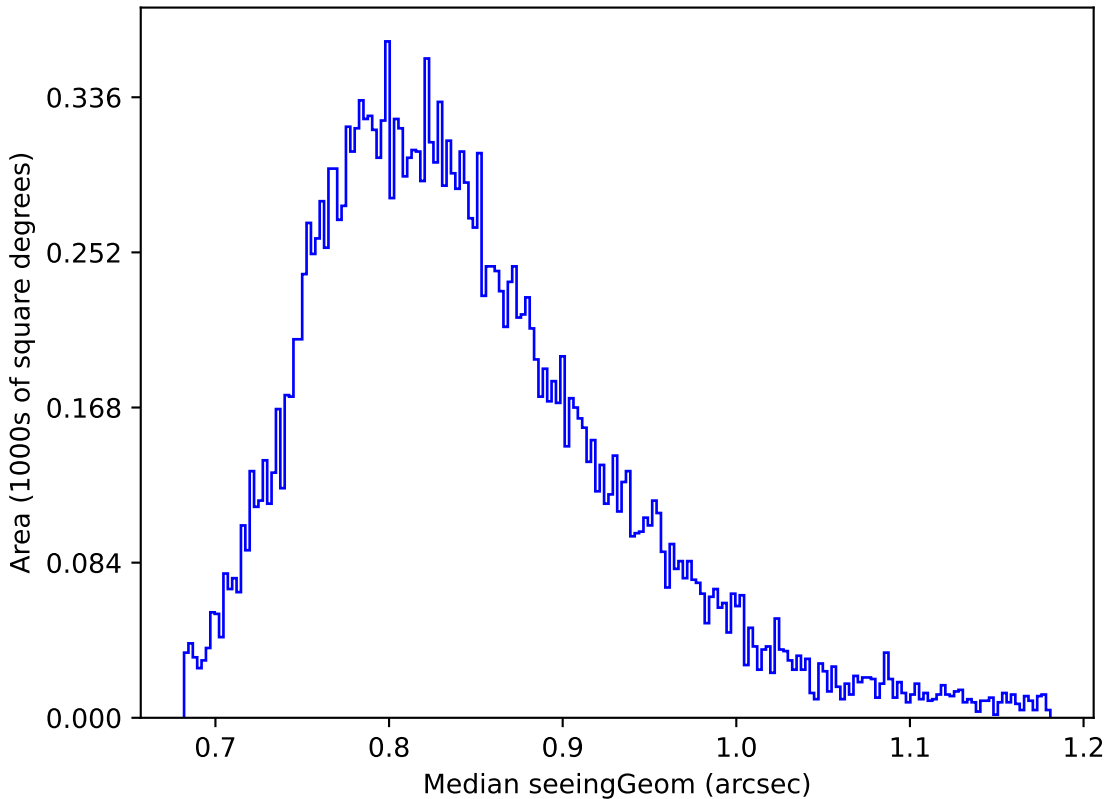
baseline_v3.5_10yrs Yr 1 y band: Median seeingGeom
