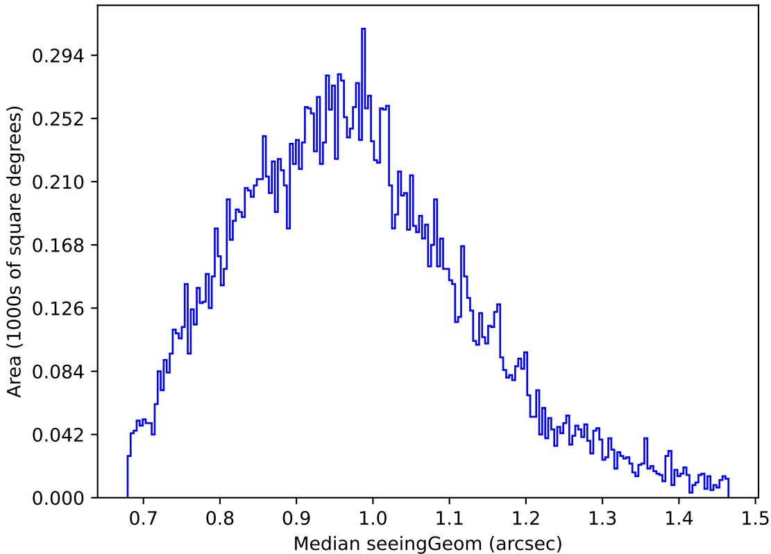
baseline_v3.5_10yrs Yr 1 u band: Median seeingGeom
