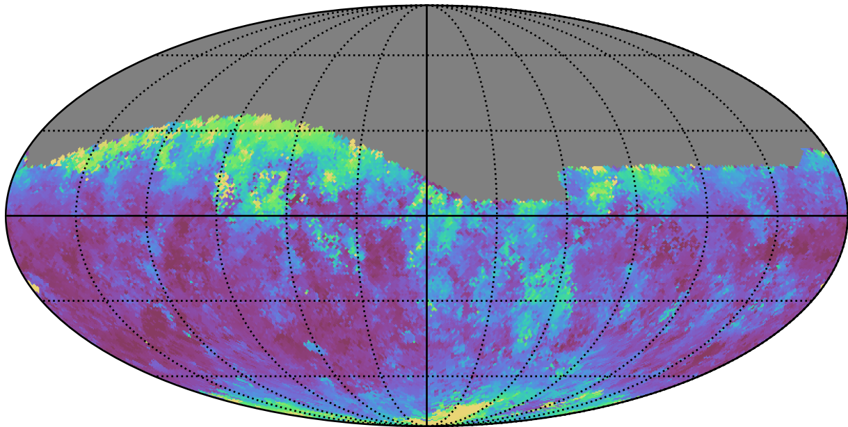
baseline_v3.5_10yrs Yr 1 r band: Median seeingGeom
