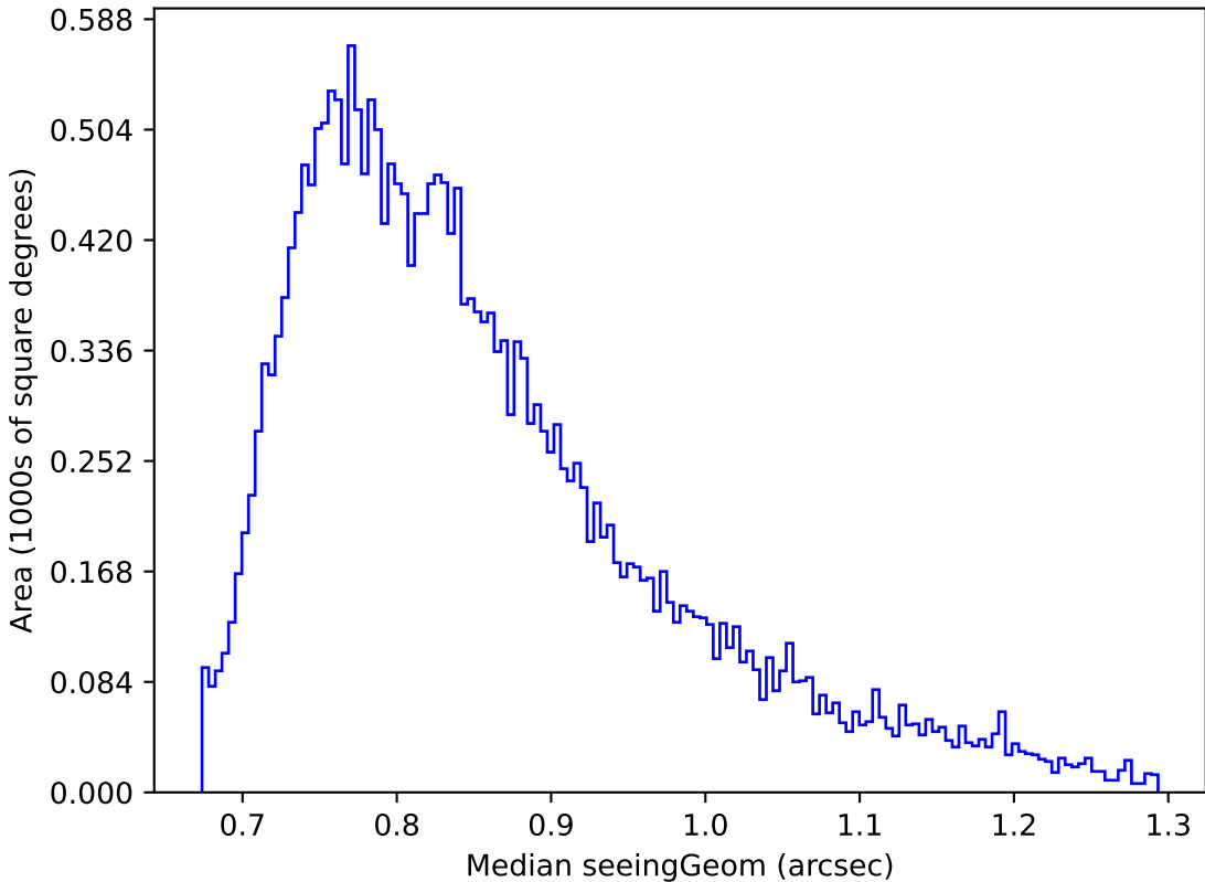
baseline_v3.5_10yrs Yr 1 r band: Median seeingGeom
