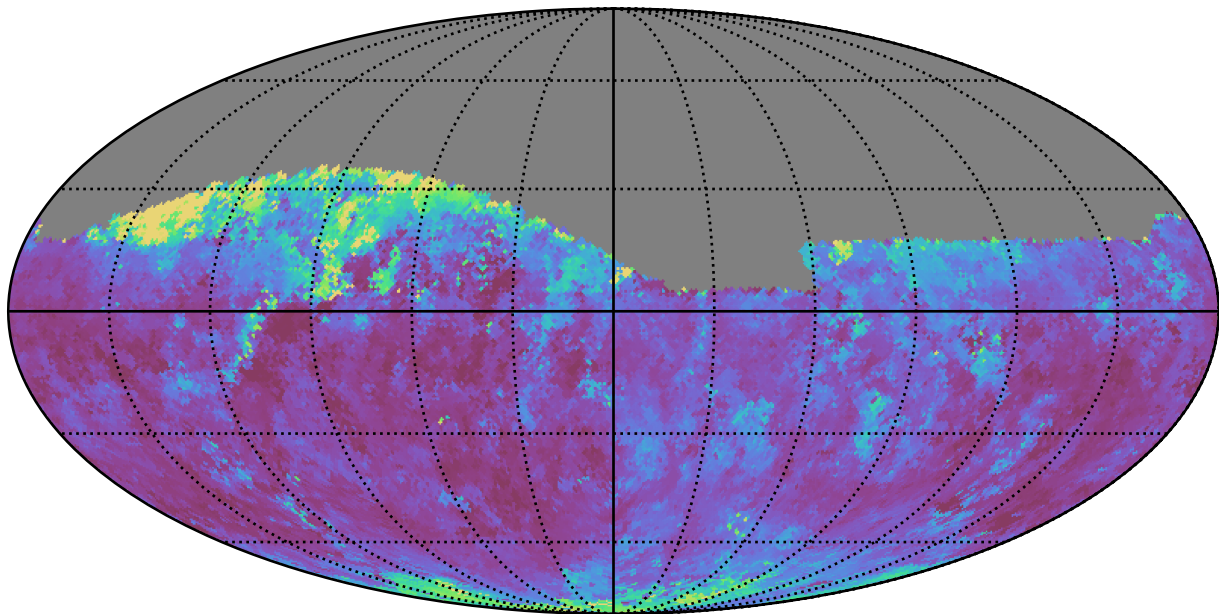
baseline_v3.5_10yrs Yr 1 i band: Median seeingGeom
