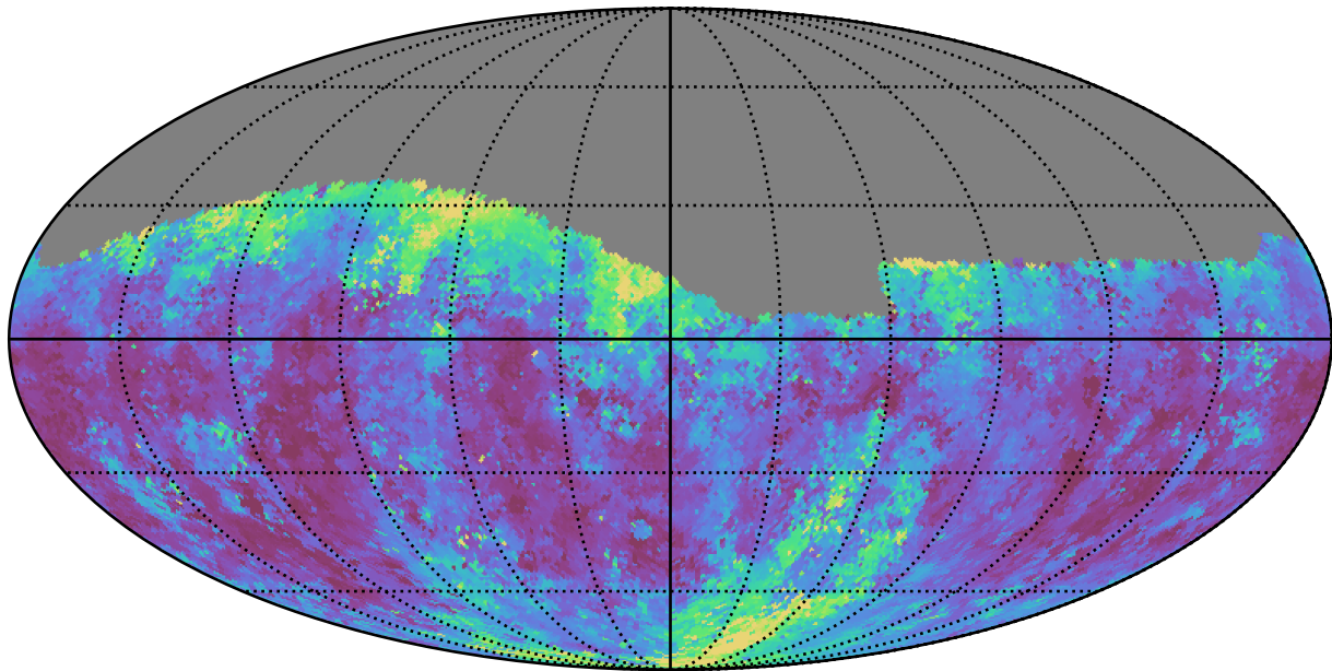
baseline_v3.5_10yrs Yr 1 g band: Median seeingGeom
