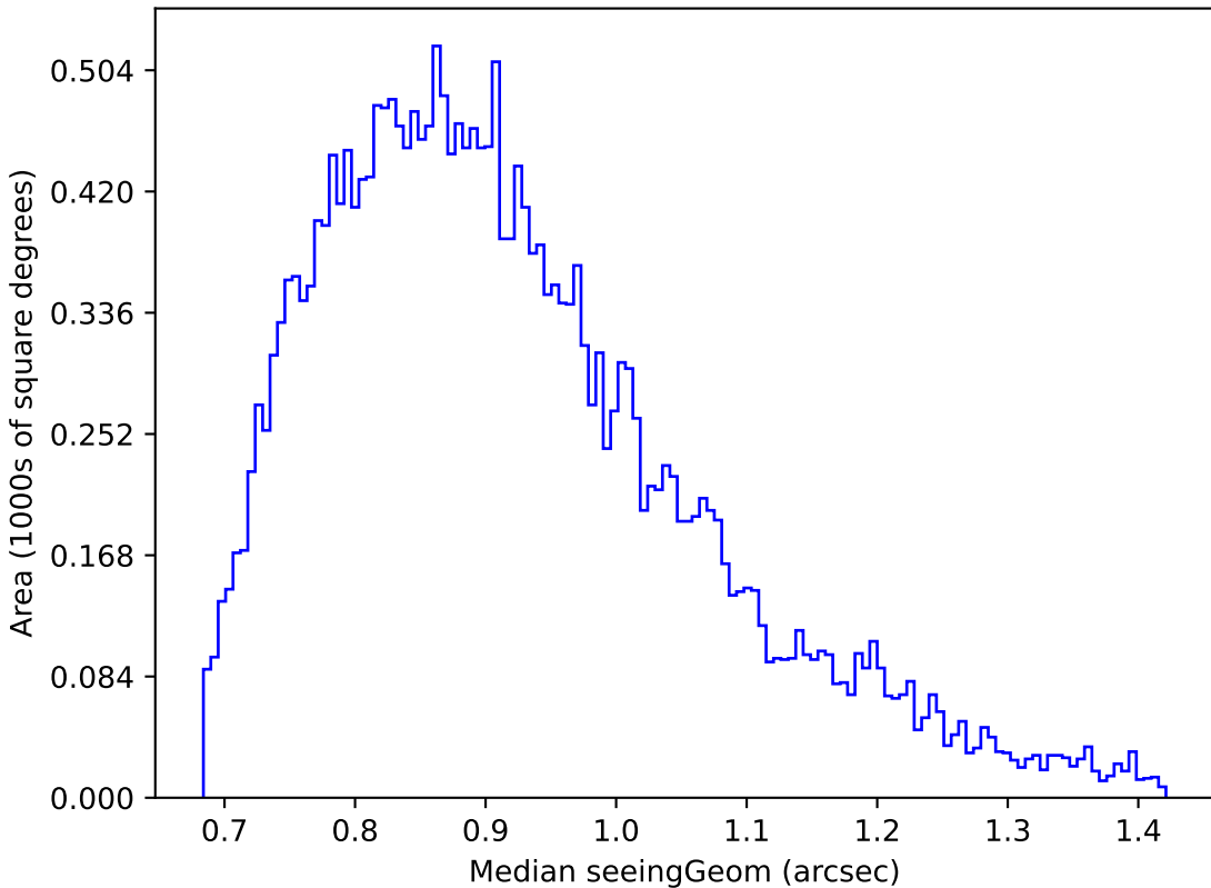
baseline_v3.5_10yrs Yr 1 g band: Median seeingGeom
