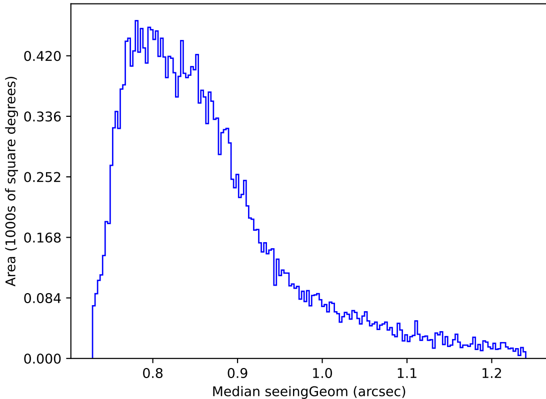
baseline_v3.5_10yrs Yr 1 all bands: Median seeingGeom
