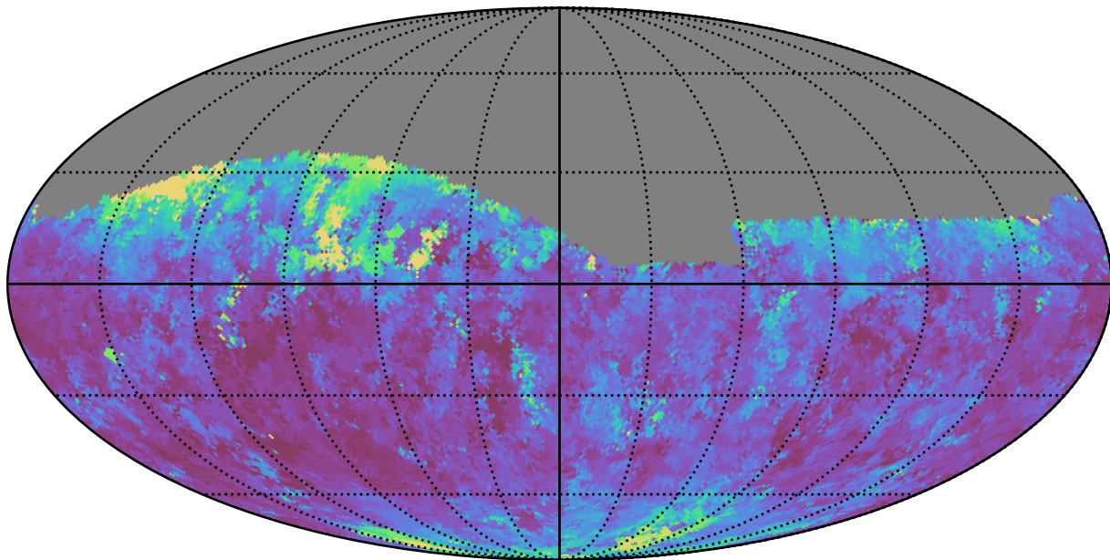
baseline_v3.5_10yrs Yr 1 z band: Median seeingEff
