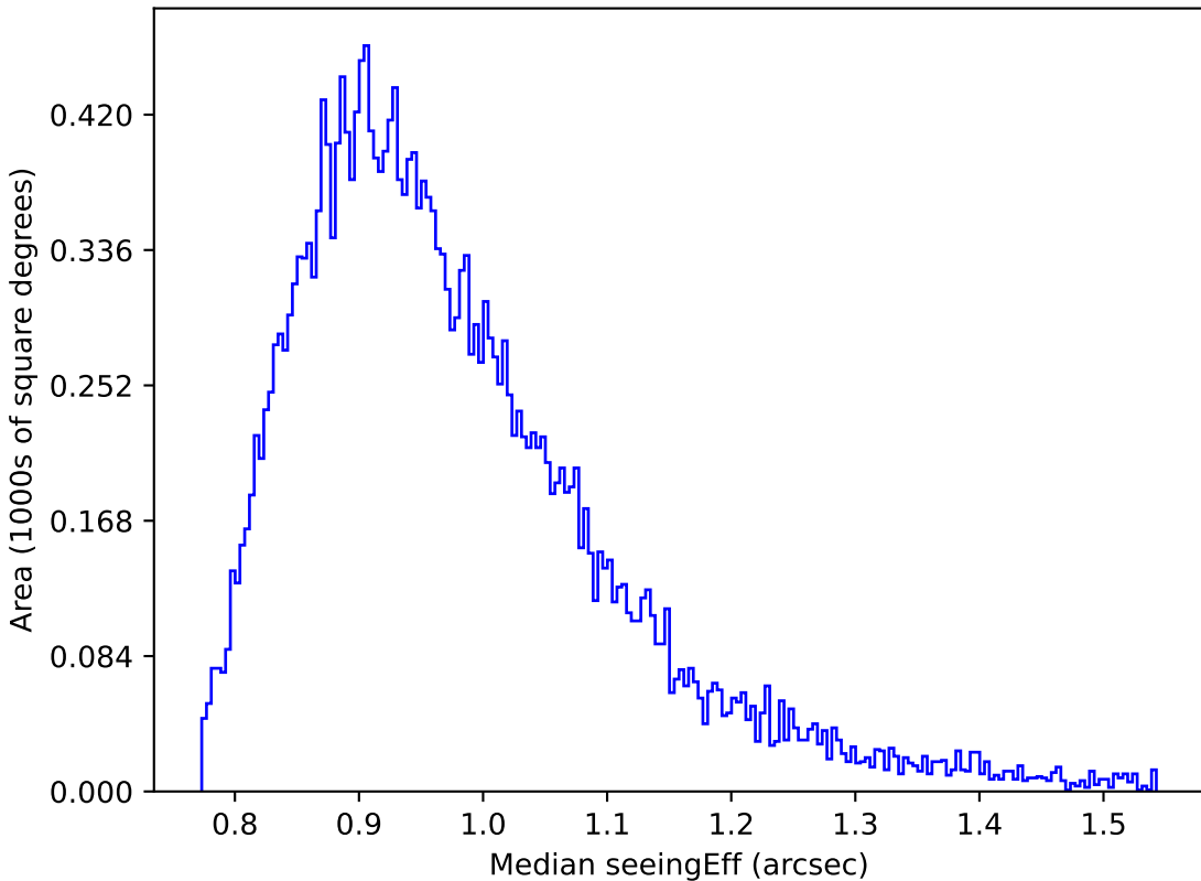
baseline_v3.5_10yrs Yr 1 z band: Median seeingEff
