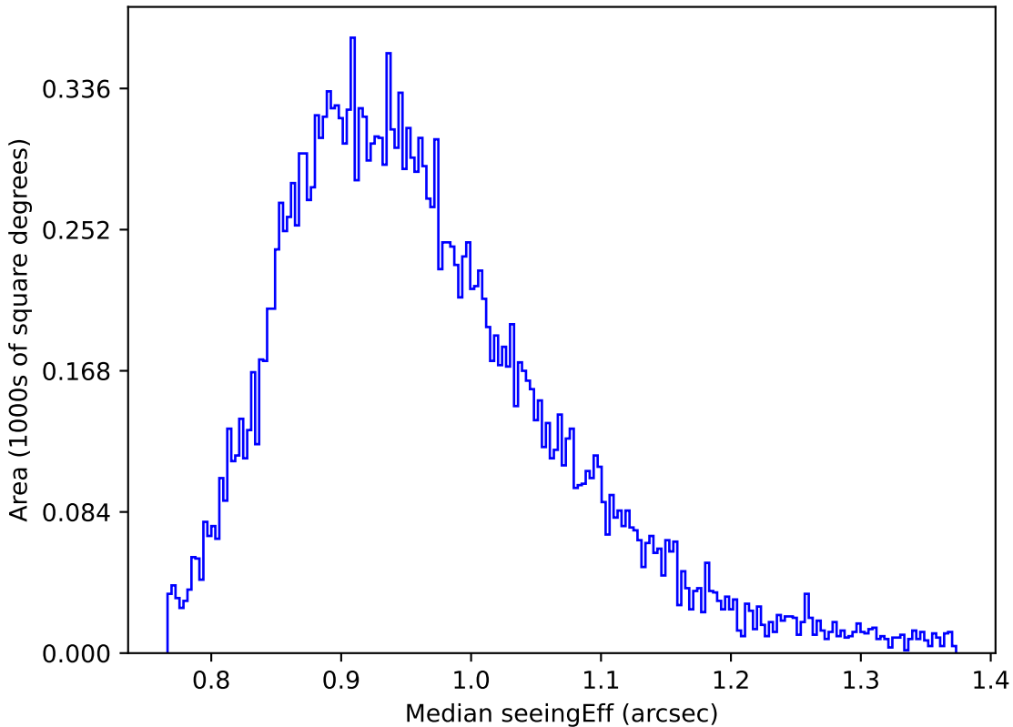
baseline_v3.5_10yrs Yr 1 y band: Median seeingEff
